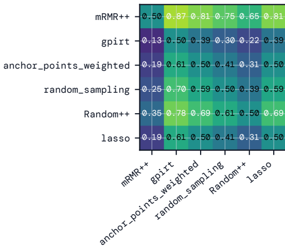
(c) Kendall \tau pairwise
